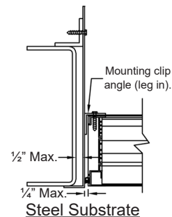
Steel Substrate
